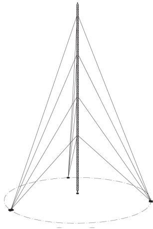
Turret base foundation ground plate (Central node) and guy wires foundation ground plates (intermediate/external node).
